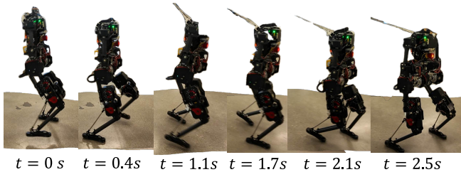
Fig. 8: BRUCE RL policy locomotion on slippery smooth concrete surface. A safety leash is attached on top at loose.
