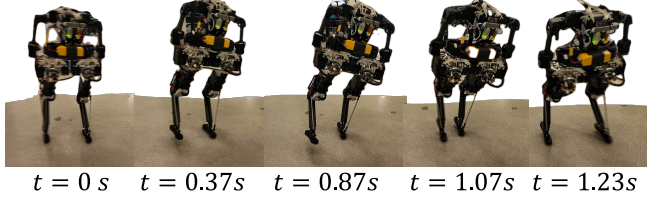
Fig. 9: BRUCE RL policy stand still perturbation rejection in sideways. BRUCE (facing backward) was able to balance on only its right leg to stabilize itself, and then took one step back. After t = 0 to t = 1.07 s the left leg was in the air. A safety leash is attached on top at loose.
