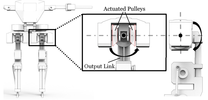
Fig. 3: The BRUCE’s cable-driven differential pulley in close up.
