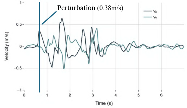
Fig. 10: Perturbation disturbance rejection from stand still. The graph shows the linear velocity odometry over time. The robot was pulled forward ( x -axis direction) at 0.38 m/s at t = 0.66 s. The robot took steps to stabilize the torso orientation.
