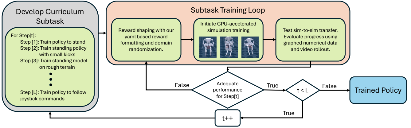
Fig. 6: Curriculum reinforcement learning framework overflow.
